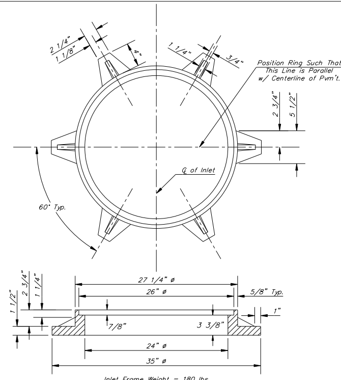
MANHOLE RING AND COVER
