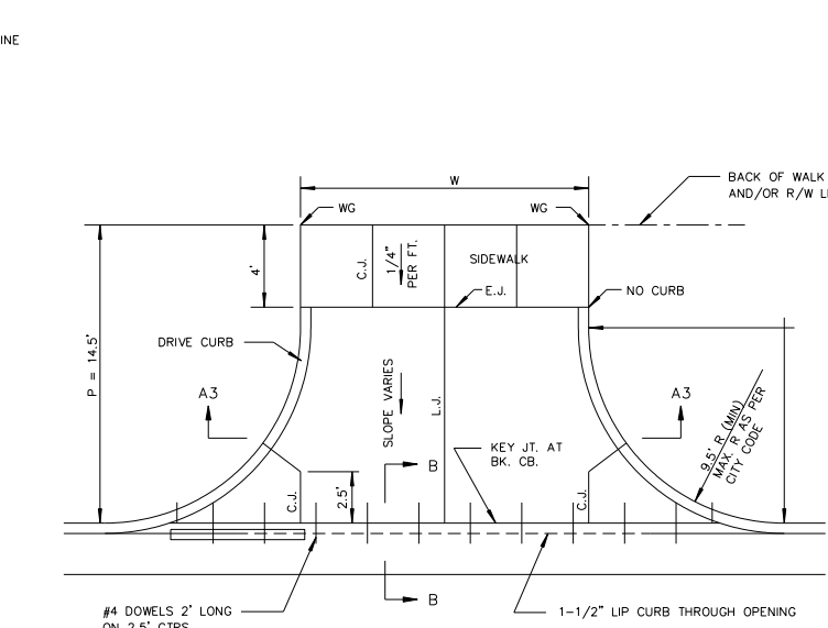
CONTRACTION JOINT (C.J.) OR LONGITUDINAL JOINT (L.J.)
