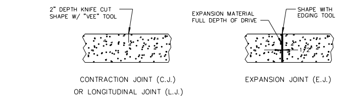
CONTRACTION JOINT (C.J.) OR LONGITUDINAL JOINT (L.J.)
